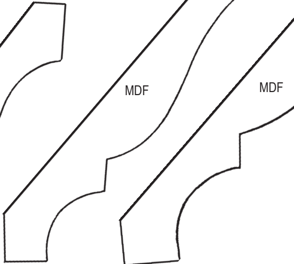
CROWN MOLD 5/8 X 4-1/4
