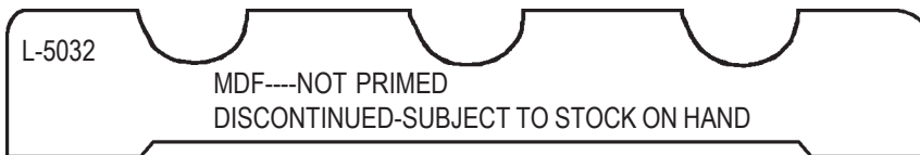
CROWN MOLD 5/8 X 4-1/4
